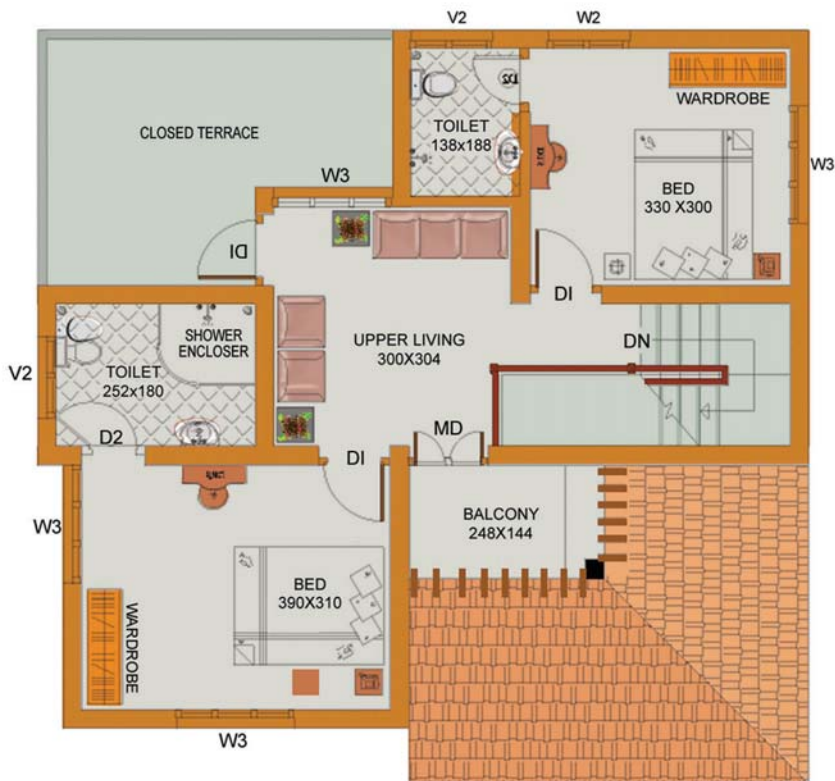
First Floor (777 Sq. Ft.)
